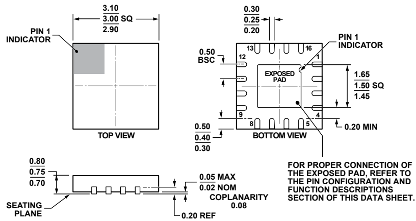
Figure 57. 16-Lead Lead Frame Chip Scale Package [LF CSP_WQ] 3 mm × 3 mm Body, Very, Very Thin Quad (CP-16-27) Dimensions shown in millimeters
