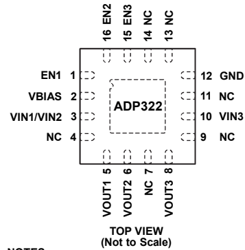
Figure 3. ADP322 Pin Configuration
